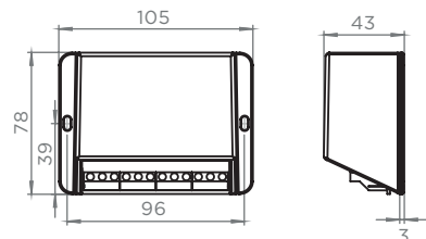
Electronic control box for Premium and Luxe systems
