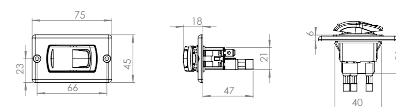
Electric switch COMFORT
